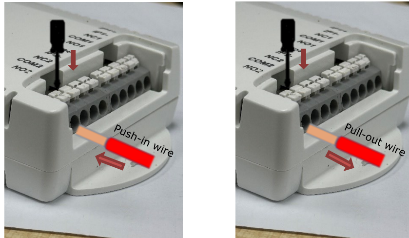
Figure 8 - Push-in wire & Pull-out wire
