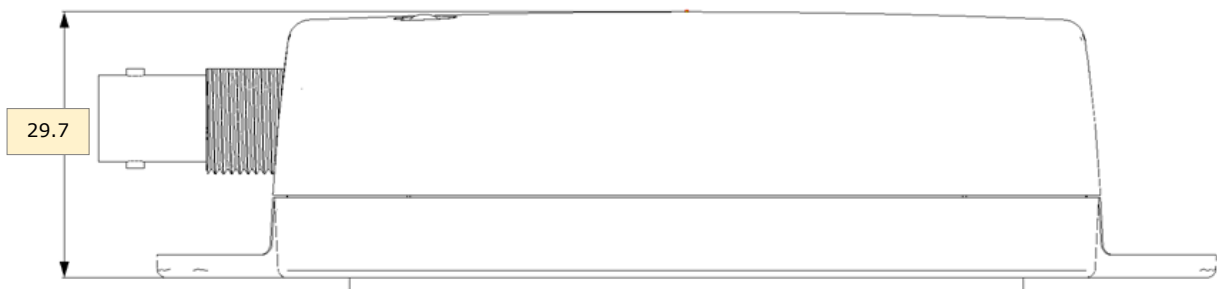
Figure 7 - Modbus Salinity Sensor Adapter Dimension – Side View
