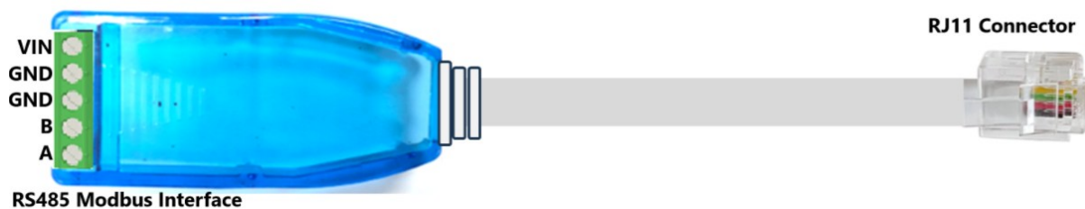
Figure 5 - RS485-RJ11 Cable(30cm)
