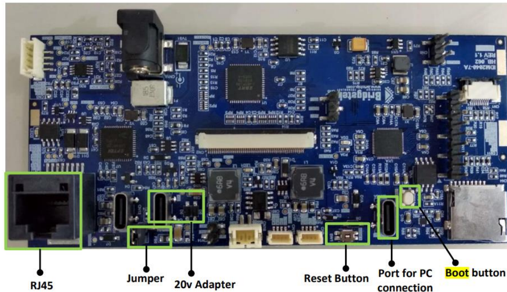
Figure 3 - IDM2040 Hardware Features
