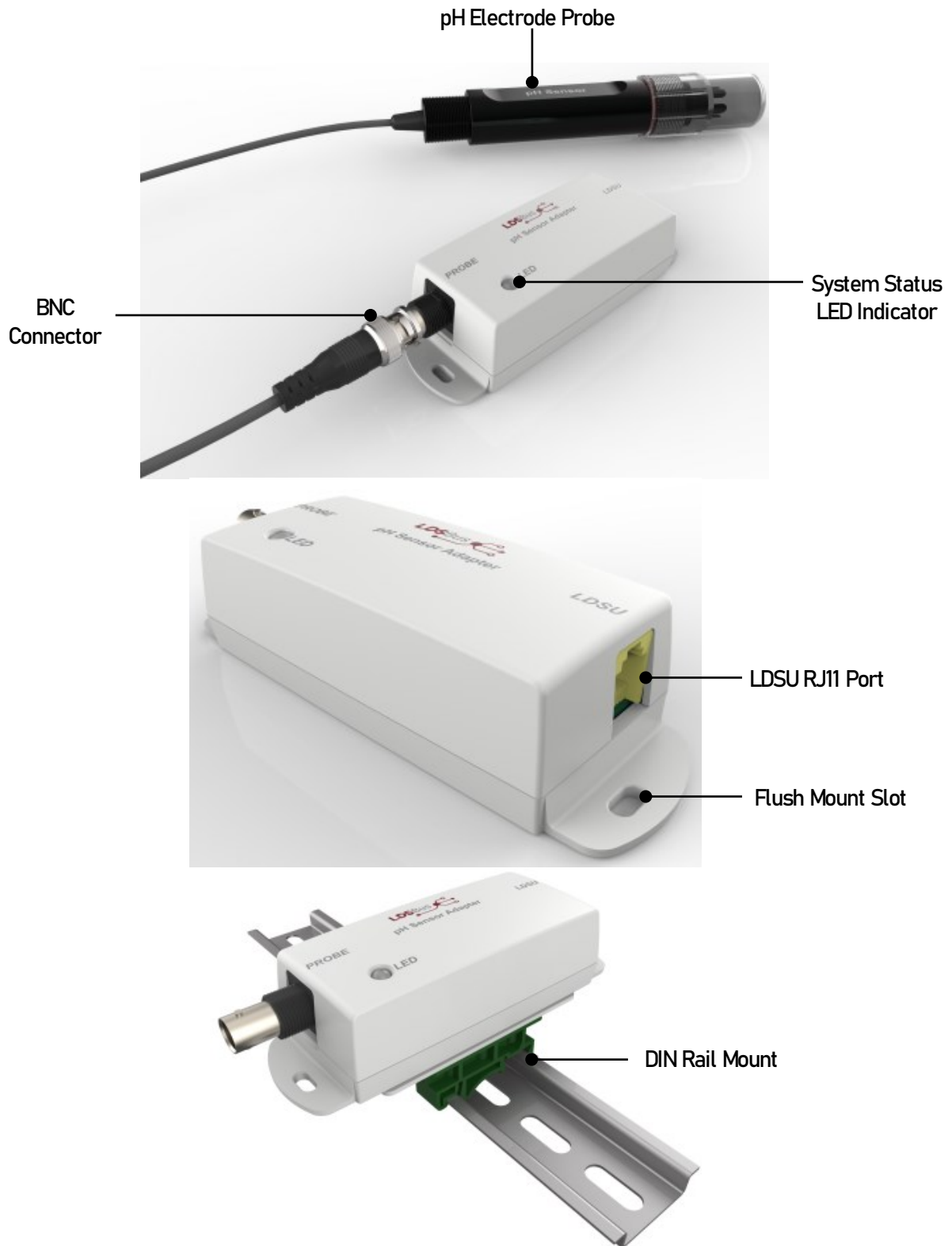
Figure 1 - LDSBus pH Sensor Adapter Hardware Features
